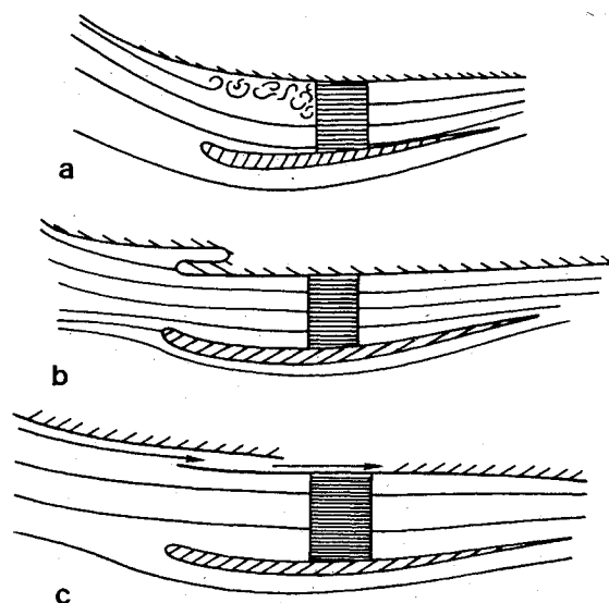
Fig. 6 Underslung inlet installation: a) airframe surface boundary-layer separation; b) offset from airframe boundary layer; and c) diversion of airframe boundary layer.
